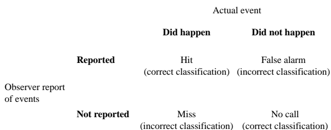
Figure 1. Signal detection model of observer accuracy
